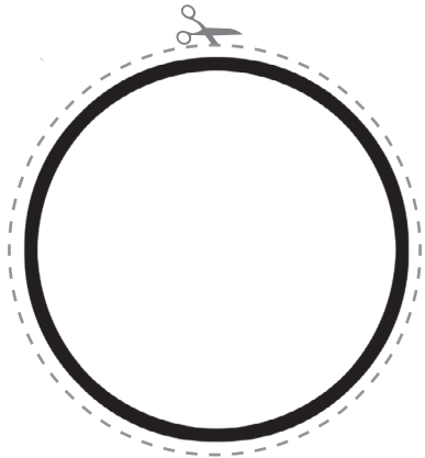
Neptune
